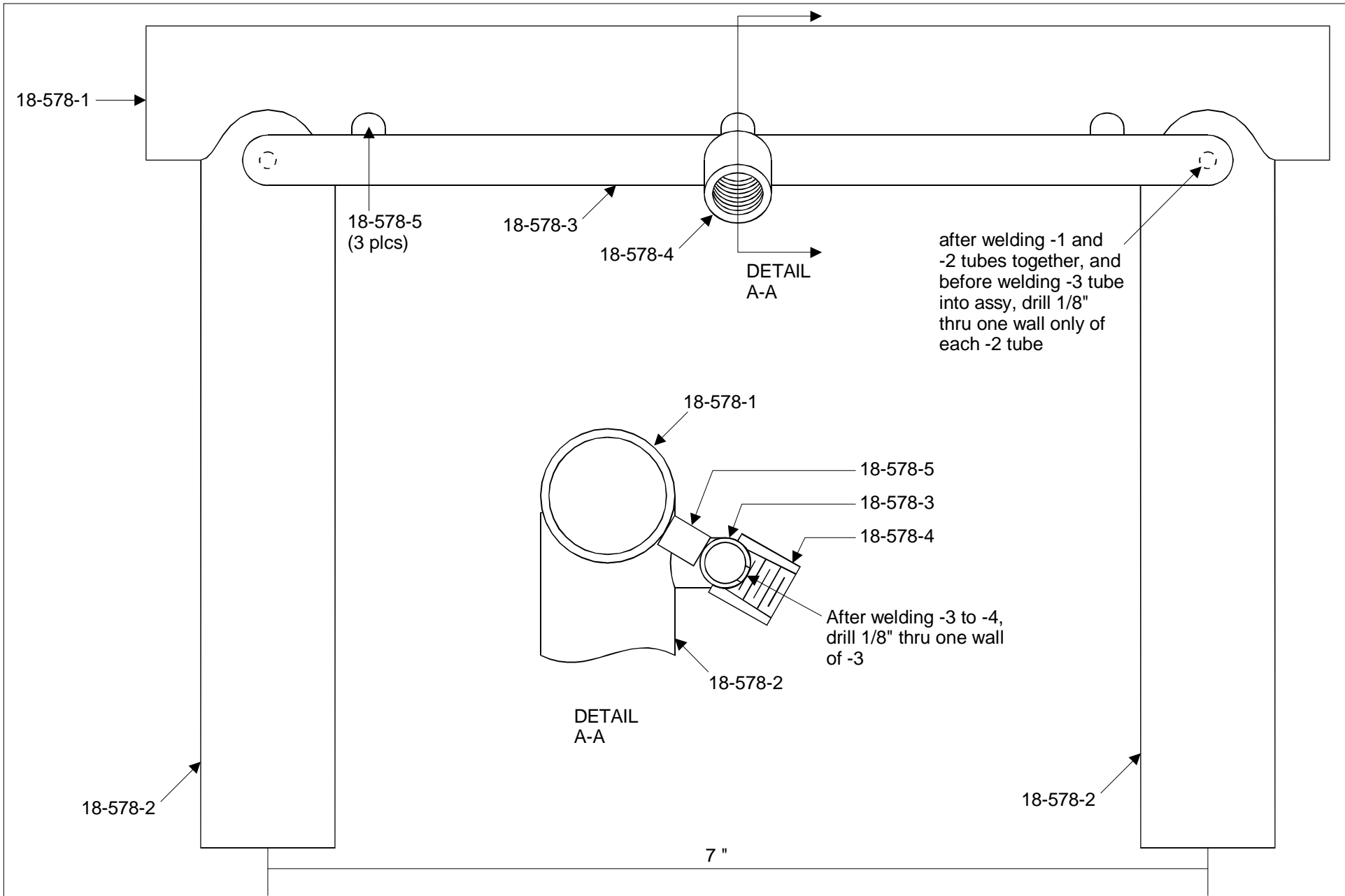
18-578 Landing Gear Upper Frame weldment assembly drawing copyright 1999 HP Aircraft, LLC HP-18 design by Richard E. Schreder drawn 28 Sept 1999 by Bob Kuykendall
