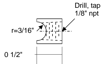
18-578-4 (1 req'd) 1/2" 4130 rod
