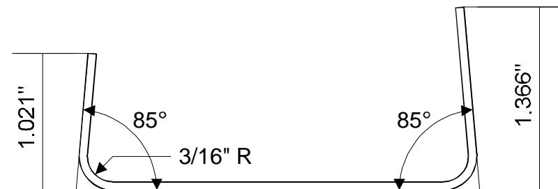
outboard end
